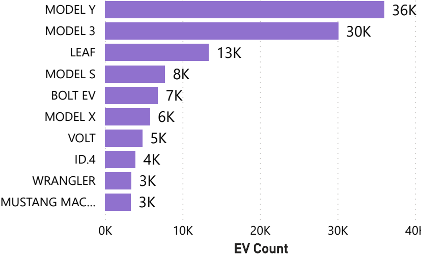
Top 10 Models
